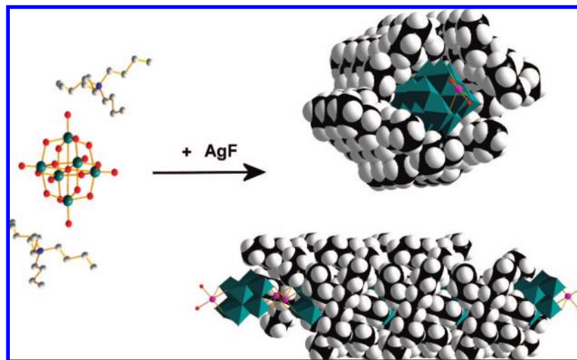
Figure 2. A schematic showing the formation of the polymeric POM architecture \text{TBA}_{2n}[\text{Ag}_2\text{Mo}_8\text{O}_{26}]_n ( 1 ) on the reaction of \text{TBA}_2[\text{Mo}_6\text{O}_{19}] with \text{AgF} . Left: \text{TBA}_2[\text{Mo}_6\text{O}_{19}] unit is shown in ball and stick representation. Color scheme: Mo, green; O, red; C, light gray; N, blue. Right: Two structural representations of 1 are shown with the silver-linked \beta -octamolybdate chain (ball and stick, and green polyhedra) wrapped in the “encapsulating” \text{TBA}^+ cations (space-filling representation). A side view along the \{\text{Ag}_2\text{Mo}_8\}_\infty chain (bottom right) and end-on view of this chain (top right) are shown. Color scheme: Mo, green polyhedra; Ag, pink; O, red; C, black; H, white.
